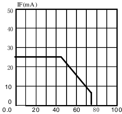
FIG.5 MAXIMUM FORWARD DC CURRENT VS AMBIENT TEMPERATURE(Tjmax=105°C)
