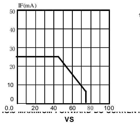
Fig.5 FORWARD CURRENT VS. AMBIENT TEMPERATURE(Tjmax=105°C)
