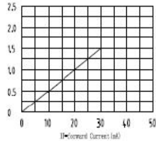
LUMINOUS INTENSITY VS FORWARD CURRENT 亮度和正向电流关系曲线图
