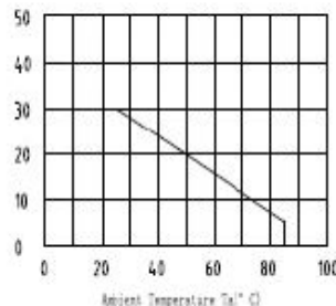
FORWARD CURRENT VS OPERATING CURRENT 正向电流随温度曲线图
