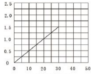
LP-forward Current (mA) LUMINOUS INTENSITY VS FORWARD CURRENT 亮度与正向电流关系曲线图
